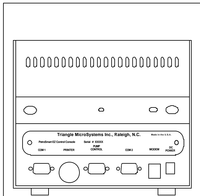
Fig. 12 , Back View of the PetroSmart EZ Console
