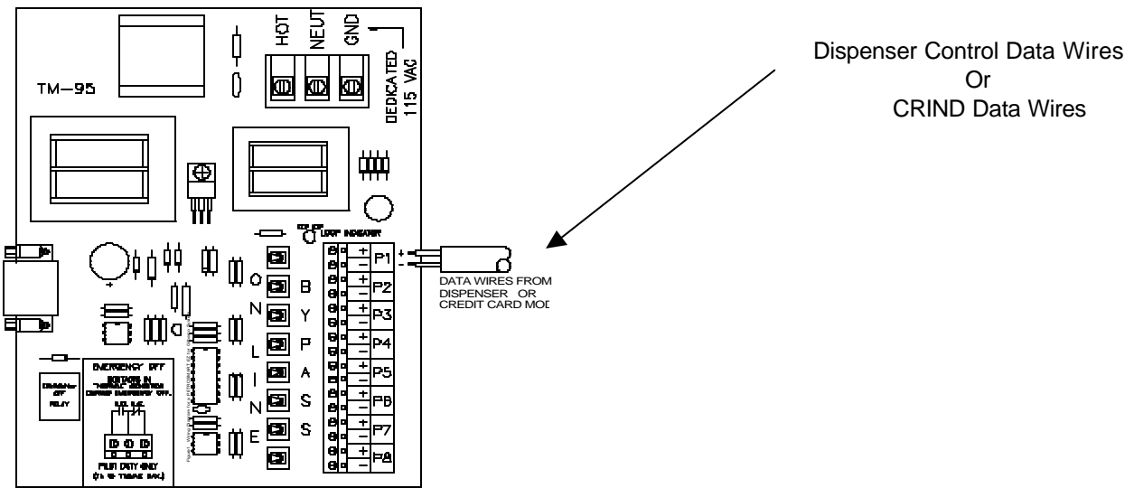
Fig. 5, Interconnect Box, MPC-TM95 Board
