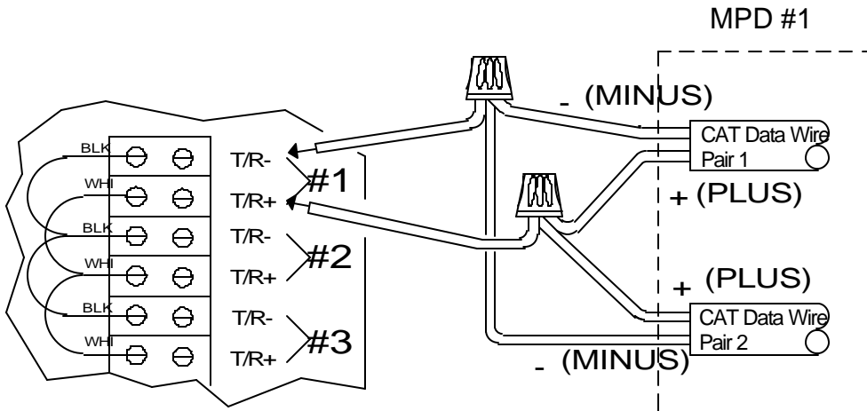
Fig. 9, How to Connect More than Eight, Dispenser Control Data wires
