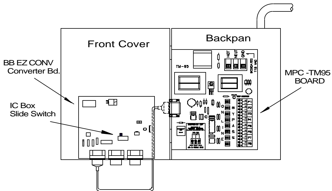
Fig. 4, The PetroSmart EZ Wayne Dispenser Control Box with the Door Open.
