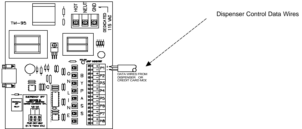
Fig. 5, Dispenser Control MPC-TM95 Board
